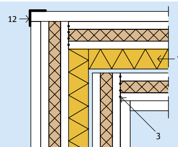
4.13.4 Hoekverbinding
