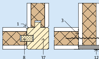
2.6.4 Hoekverbinding
